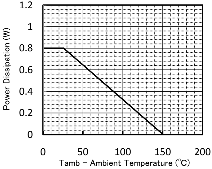
Fig. 1 – Power Dissipation Vs. Ambient Temperature
